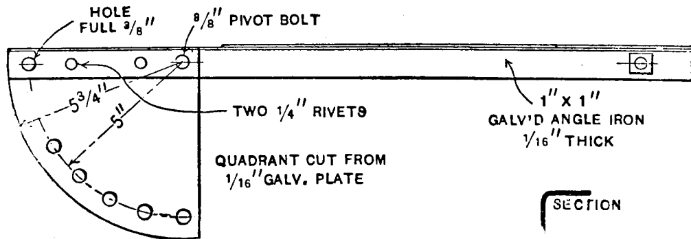
FIG. 37.—Elevation and Plan of Tail Regulator.
