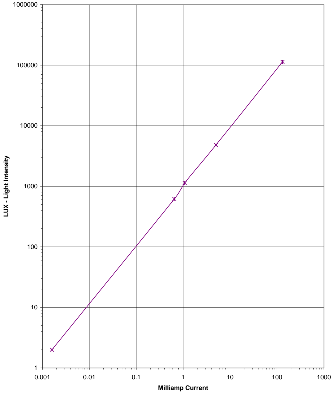
Calibration Curve for Silicon Solar Cell of 1.368 Sq. Inches using digital Amp-meter Cen-Tech P30756
