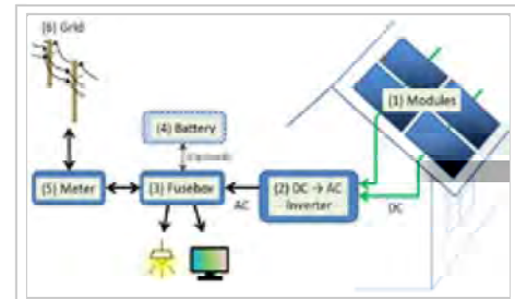
Simplified schematics of a grid-connected residential photovoltaic power system
