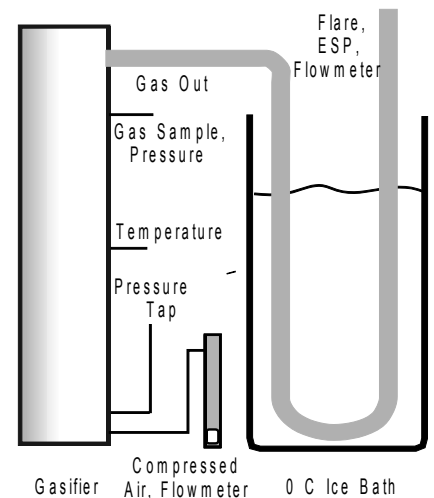
Fig. 2 - Gas Train
