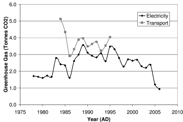
Figure 1 Greenhouse gas emission data for Sanderson household: Electricity emissions from 1978 to 2006; Transport emissions (2 cars) from 1984 to 1995.
