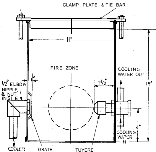
Above, Fig. 4: Distemper drum producer; and right, Fig. 5: Final design of gas producer
