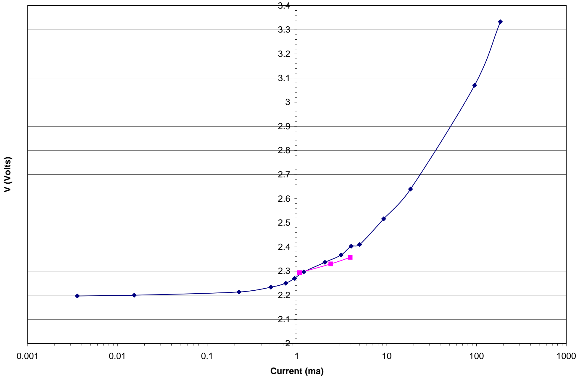
Charging Current ver Voltage for a charged cell Current flow per amp-hour battery capacity
