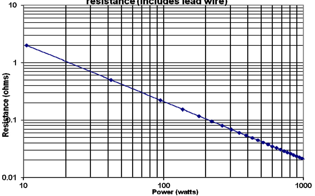
Maximum Power from battery bank of given internal resistance (includes lead wire)
